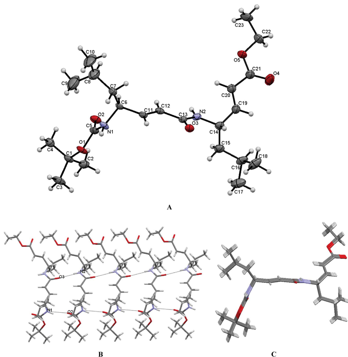
Fig. 5 Crystal structure of dipeptide Boc-dgL-dgL-OEt (D4). A. The ORTEP diagram of the dipeptide. B. The partial \beta -sheet of character exhibited by the dipeptide in crystals. C. The side view of the \beta -sheets.
