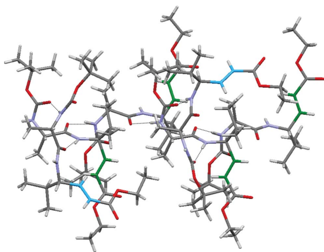
Fig. 4 Crystal structure of dipeptide Boc-Ala-dgV-OEt. Six molecules are appeared in the asymmetric unit. The intermolecular H-bonding between the dipeptide units are shown in dotted lines. The types of conformations with significant variation in the torsional values of vinyllogous residues are highlighted in different colours.
