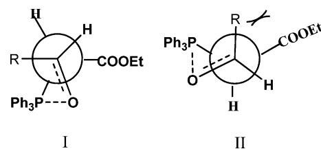
Scheme 2 Schematic representation of the transition states of the formation of E (I) and Z (II) products.
