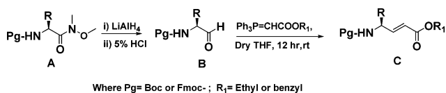
Scheme 1 Synthesis of \alpha,\beta -unsaturated \gamma -amino esters using Wittig reaction.
