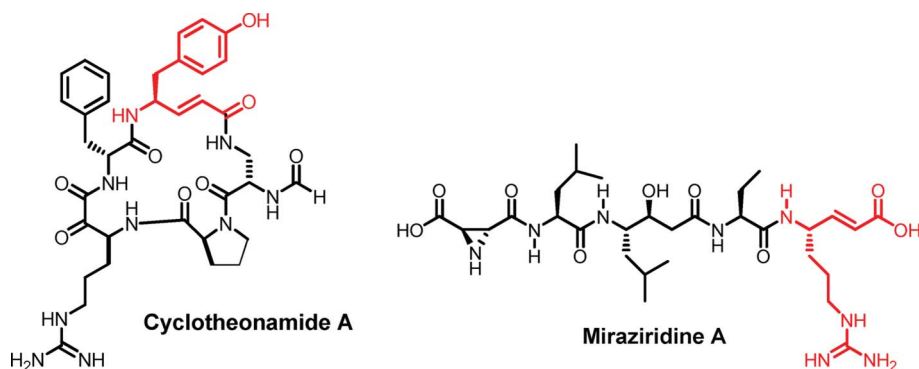
Fig. 1 Representative examples of vinylogous amino acids in peptide natural products.
