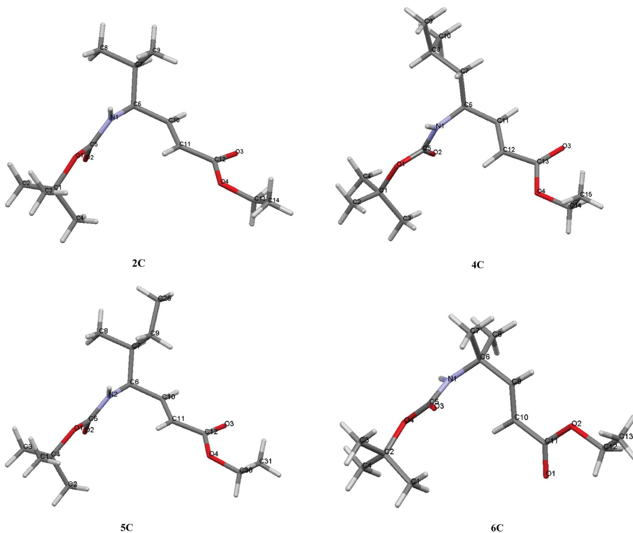
Fig. 3 Crystal structures of vinyllogous amino esters, Boc-( S, E )-dgV-OEt ( 2C ), Boc-( S, E )-dgL-OEt ( 4C ), Boc-( S, E )-dgI-OEt ( 5C ) and Boc-( E )-dgU-OEt( 6C ).
