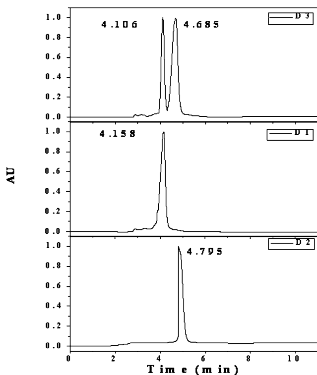
Fig. 2 Chiral HPLC of dipeptides D1 , D2 , and D3 . The HPLC was performed on Daicel CHIRALPAK-AI column using 20% isopropanol in n-hexane as a solvent system at isocratic mode with the flow rate of 1 mL/min.
